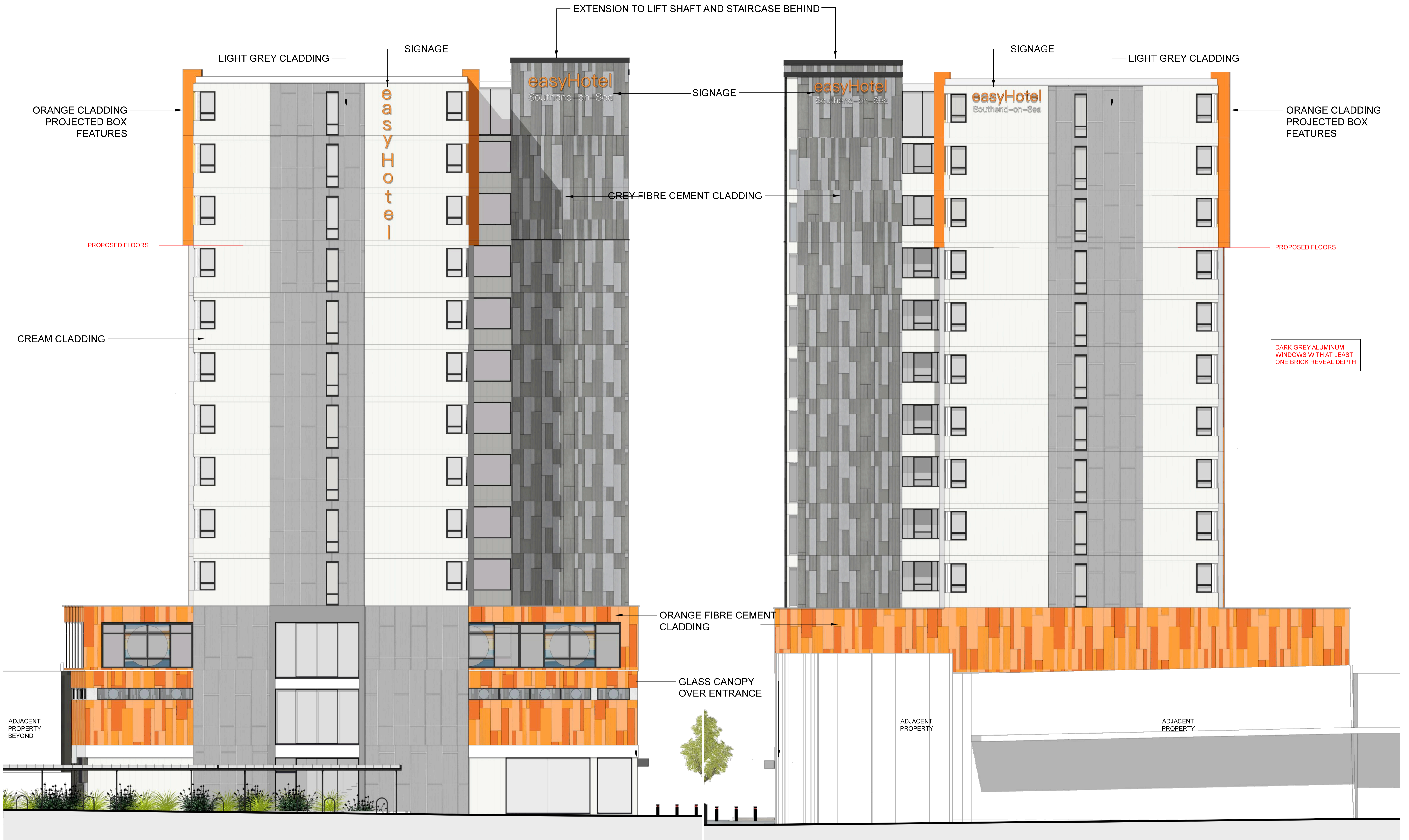
SIDE (LEFT) ELEVATION
